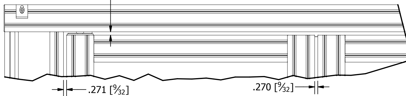
DETAIL D
