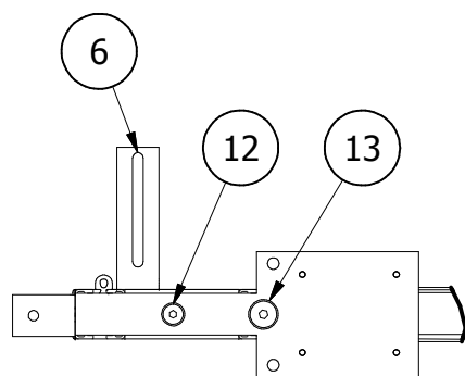
DETAIL C
